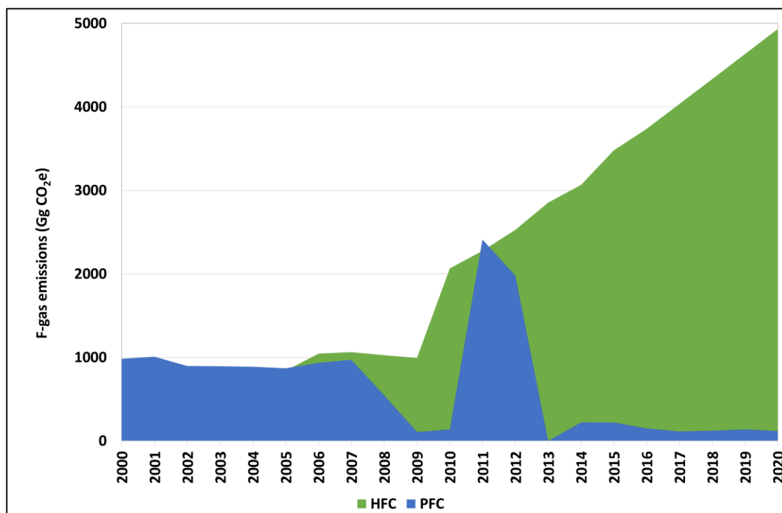
Figure 2.8: Trend in F-gas emissions in South Africa, 2000 – 2020.
