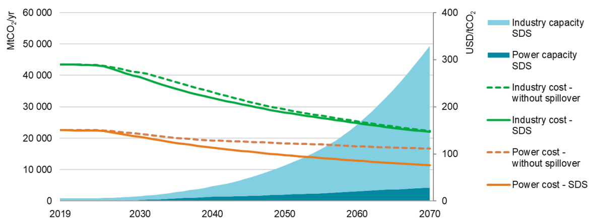
Figure 3.13 Capital cost learning curve (right) and cumulative capacity (left) for chemical absorption in industrial and power applications in the Sustainable Development Scenario
