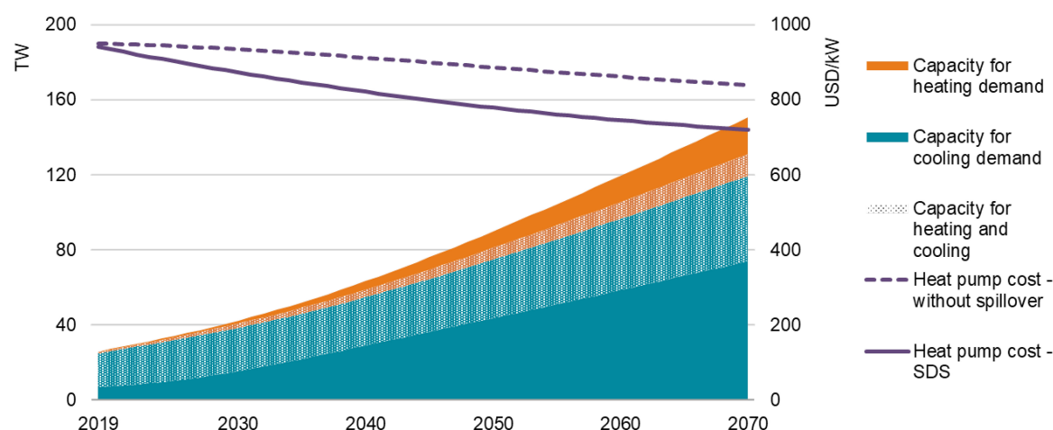
Figure 3.14 Capital cost learning curve (right) and cumulative capacity (left) for vapour compression applications in the Sustainable Development Scenario
