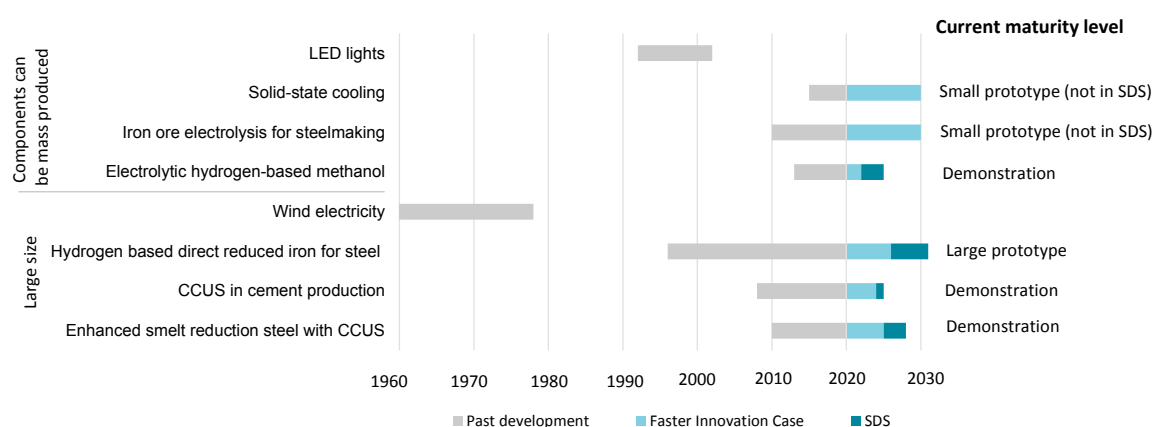
Figure 4.2 Period from first prototype to market introduction for selected technologies, including the quickest examples in recent clean energy technology development
