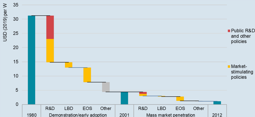
Contributions to solar PV cost declines by high-level mechanism and driver
