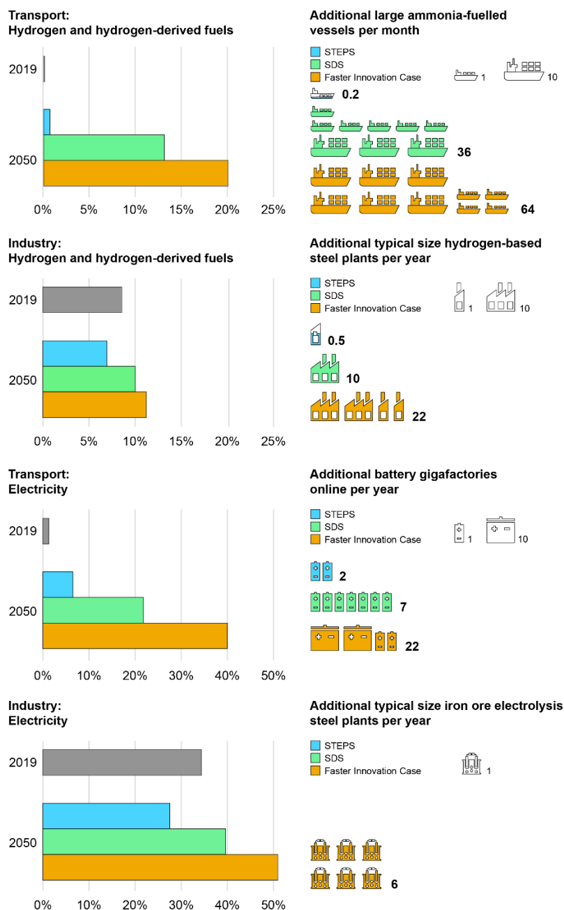
Figure 4.4 World share of hydrogen and electricity in final energy demand by end-use sector (left) and selected adoption metrics of hydrogen technologies (right)
