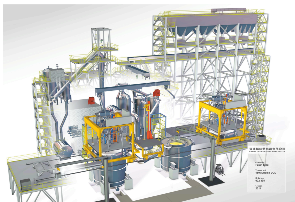
Graphic representation of the Duplex-VOD X-eeed plant at Fujian Fuxin Special Steel.
